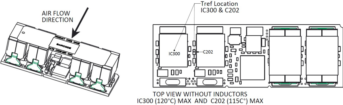
Figure 29. Preferred airflow direction and the location of the thermal reference points
