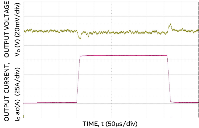
Figure 16. Trans. Resp. to 100A/μs Load Change from 25% to 75% at 12V IN , C o =4x0.047μF + 4x0.1μF + 15x22μF + 73x47μF + 6x470μF polymer.
