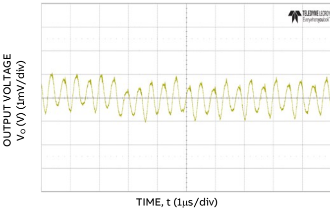
Figure 15. Typical output ripple (C o =4x0.047μF + 4x0.1μF + 15x22μF + 73x47μF + 6x470μF polymer, V IN = 12V, I o = I o,max ).
