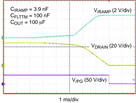
Figure 12. \overline{\text{P}}\text{G} Output Timing - Voltage Qualified
