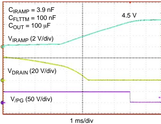
Figure 13. \overline{\text{P}}\text{G} Output Timing - Current Qualified
